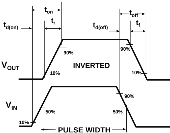
Figure 2. Switching Waveforms
