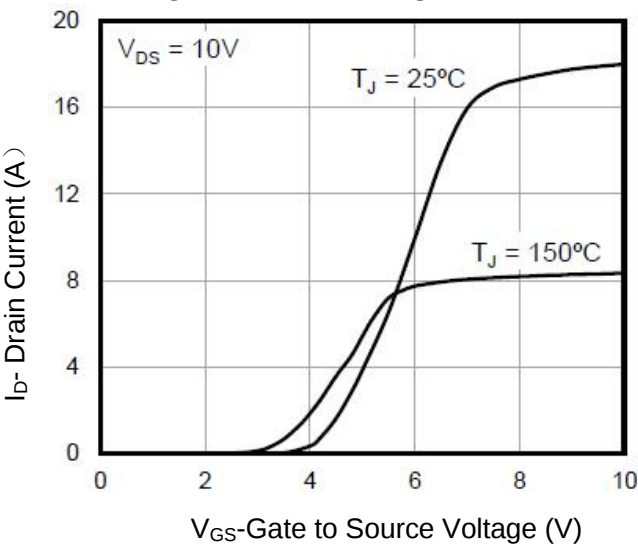
Figure 4. Transfer Charateristics
